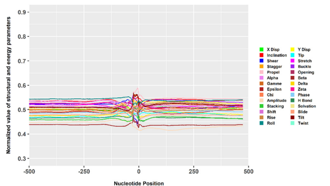
Fig. 6 Normalised and combined structure and energy graph for all sequences (197 356) containing TSS from the 8 eukaryotic species.
