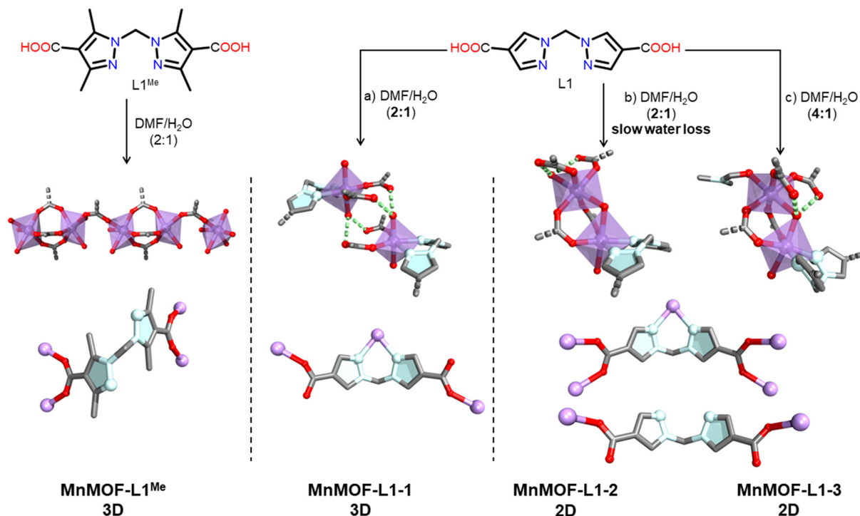
Fig. 3 Synthesis conditions and key structural features of materials made from the shorter linkers, L1 Me and L1. Subtle variations in the DMF : water ratio and rate of water loss dictate the formation of three different phases for L1. From left to right, crystallographic representations of the Mn(II) clusters and ligand connectivities of MnMOF-L1 Me , MnMOF-L1-1, MnMOF-L1-2 and MnMOF-L1-3 (C, grey; N, light blue; O, red; Mn, purple). Hydrogen atoms have been omitted for clarity.
