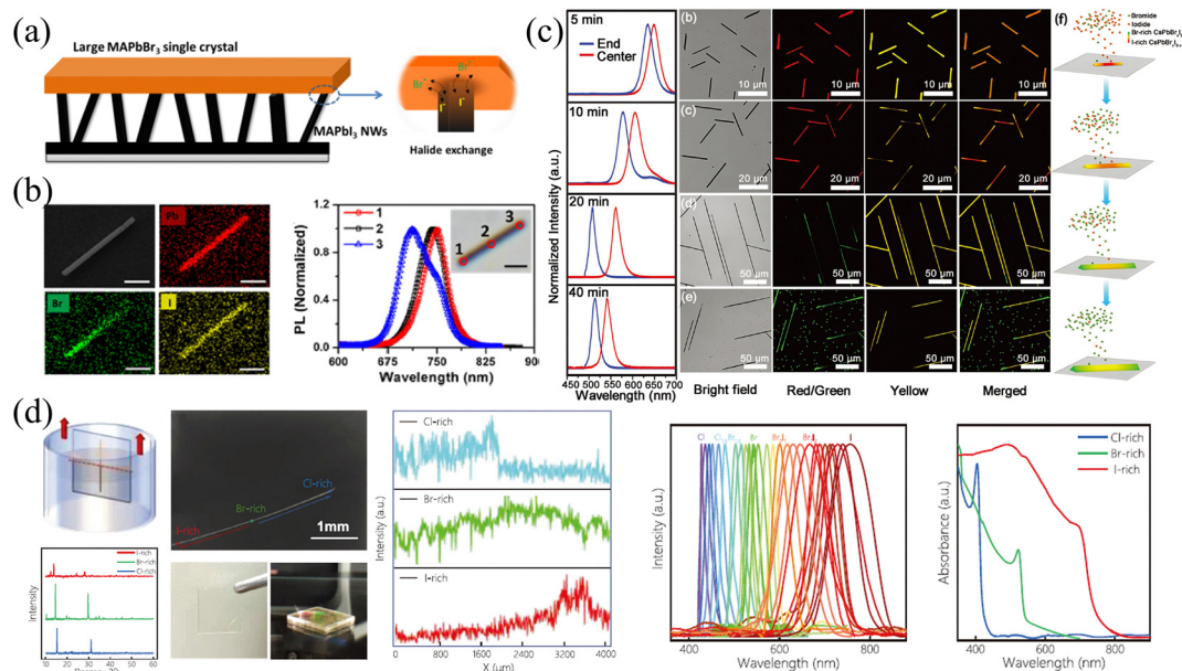
Fig. 10 (a) Schematic diagram of solid-phase ion exchange for HP NWs. (b) EDS mappings and PL spectra at different regions of compositional gradient \text{MAPbBr}_{x-1}\text{I}_{3-x} NWs. (a) and (b) Reprinted with permission from ref. 77, Copyright 2017, American Chemical Society. (c) PL spectra at the end and center of \text{CsPbBr}_{x-1}\text{I}_{3-x} NWs at different reaction times, and corresponding confocal laser scanning microscope image and schematic diagram of the growth process of compositional gradient \text{CsPbBr}_{x-1}\text{I}_{3-x} NWs. Reprinted with permission from ref. 89, Copyright 2018, John Wiley and Sons. (d) Schematic diagram of the dip-and-pull method for liquid-phase ion exchange for MWs, and corresponding characterization of the compositional gradient MWs. Reprinted with permission from ref. 41, Copyright 2022, John Wiley and Sons.
