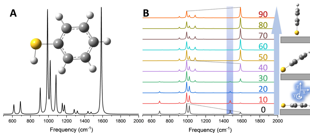
Fig. 1 (A) Ensemble averaged Raman spectrum of an isolated TP molecule computed at the B3LYP/6-311+G** level of theory. (B) Molecular orientation-dependent Raman scattering from TP, simulated following eqn (5) in the main text with incident and scattered fields along Z . The spectra were obtained by rotating the molecule around Y (see the lower right inset of panel B, and the color coded numbers correspond to rotation angles in degrees). The inset shows a schematic representation of the molecule atop the surface in the laboratory frame. All spectra were scaled with a single factor of 0.975. The orientation-dependent spectra were otherwise individually normalized.
