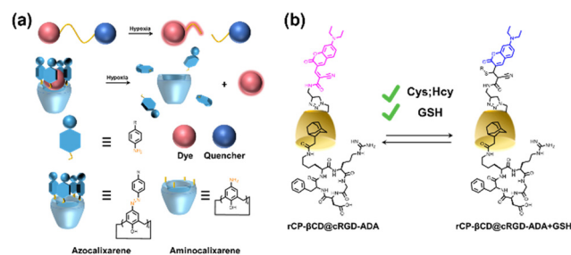
Fig. 8 (a) Schematic illustration of the design principles of the conventional covalent and the proposed noncovalent strategies for creating hypoxia-responsive systems. (b) Construction of rCP-βCD@cRGD-ADA and the reversible Michael addition reactions between rCP-βCD@cRGD-ADA and biothiols.
