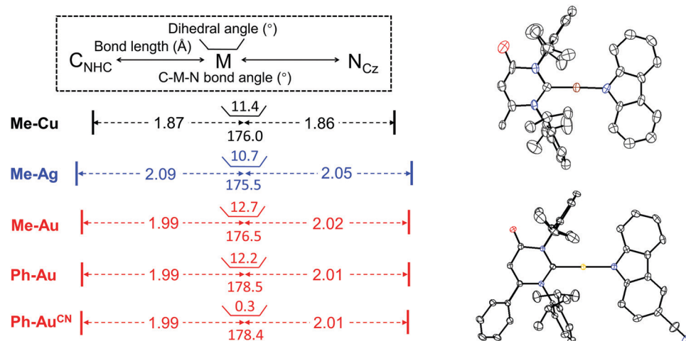
Fig. 2 Critical crystallographic data from X-ray single crystal diffraction measurements, C NHC denotes the carbene carbon and N Cz is the carbazolyl nitrogen. Thermal ellipsoid figures of Me-Cu (top) and Ph-Au CN (bottom).
