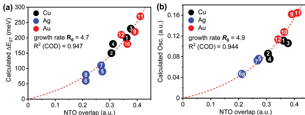
Fig. 5 Relationship between ^1\text{ICT} NTO overlap value versus theoretically calculated (a) \Delta E_{\text{ST}} and (b) oscillator strength of the S_1 state by the TD-DFT method; fits to the data are obtained using the exponential growth function: y = A(e^{R_0 x} - 1) .
