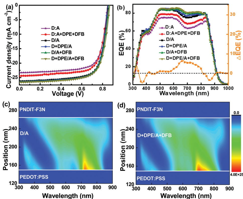
Fig. 2 BHJ and LbL-PSCs prepared without or with solvent additives: (a) The J - V curves, (b) the EQE spectra and the \Delta\text{EQE} between the additive-processed LbL devices and the control one. (c) Photogenerated exciton distribution in PNTB6-Cl/Y6 layers, and (d) photogenerated exciton distribution in PNTB6-Cl + DPE/Y6 + DFB layers.
