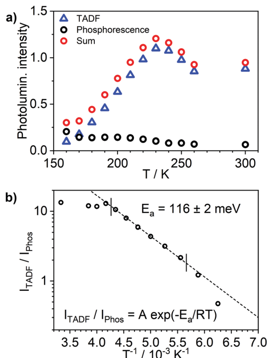
Fig. 4 Photoluminescence of complex 3 in toluene solution ( c = 10^{-5} \text{ M} ) as a function of temperature: (a) intensity of TADF, intensity of phosphorescence and their sum (total intensity); (b) ratio of TADF to phosphorescence.
