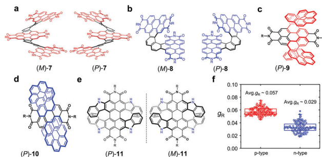
Fig. 4 (a)–(e) Molecular structure of PDI-helicenes (M/P)-7, (M/P)-8, (P)-9, (P)-10, and (P/M)-11. Reproduced with permission from ref. 36. Copyright 2018, American Chemical Society. (P)-9, (P)-10, Reproduced with permission from ref. 40. Copyright 2020, American Chemical Society and (P/M)-11; (f) quantitative analysis results of g_R of four (P)-11 OFET devices under CPL irradiations ( \lambda = 635 nm). Reproduced with permission from ref. 41. Copyright 2021, Nature Publishing Group.
