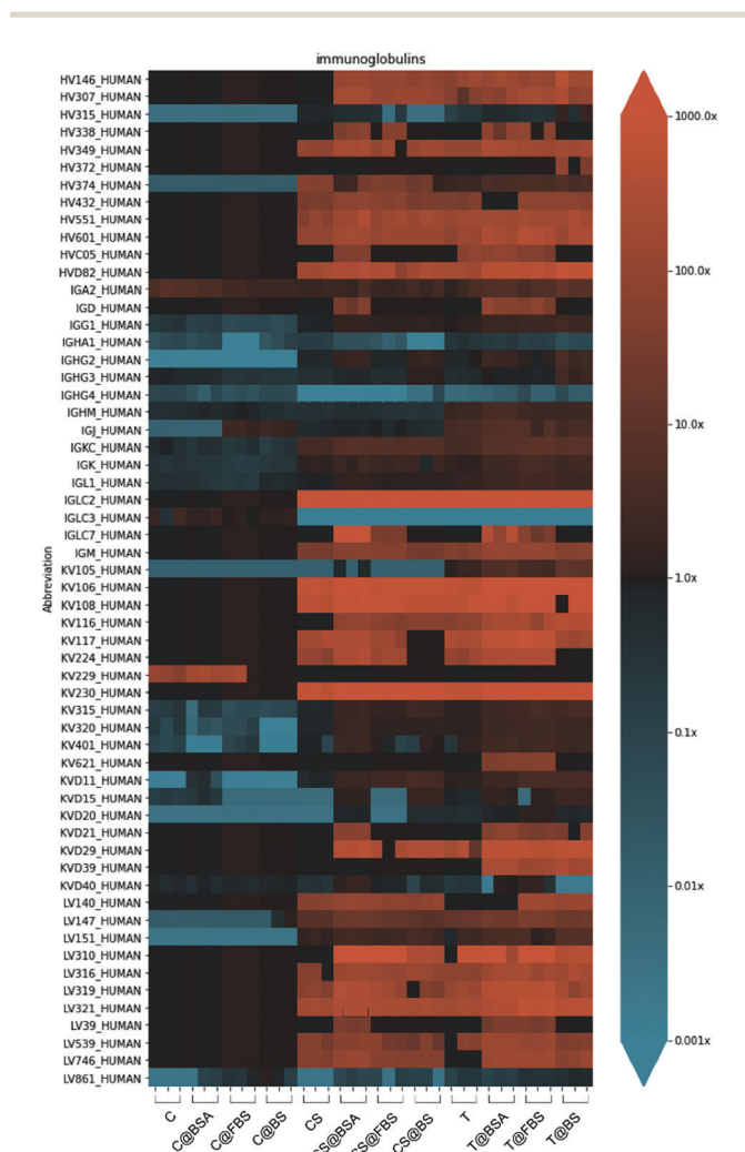
Fig. 6 Heatmap of the differential enrichment of immunoglobulins in the biomolecular coronas of the Au@BDT templates (T, T@BSA, T@FBS, and T@BS), Au@BDT@MPN core-shell nanoparticles (CS, CS@BSA, CS@FBS, and CS@BS), and Au@MPN nanocapsules (C, C@BSA, C@FBS, and C@BS) without and with pre-coating. The proteins are listed alphabetically in a colorized log scale. Three replicates of each nanoparticle system were examined.
