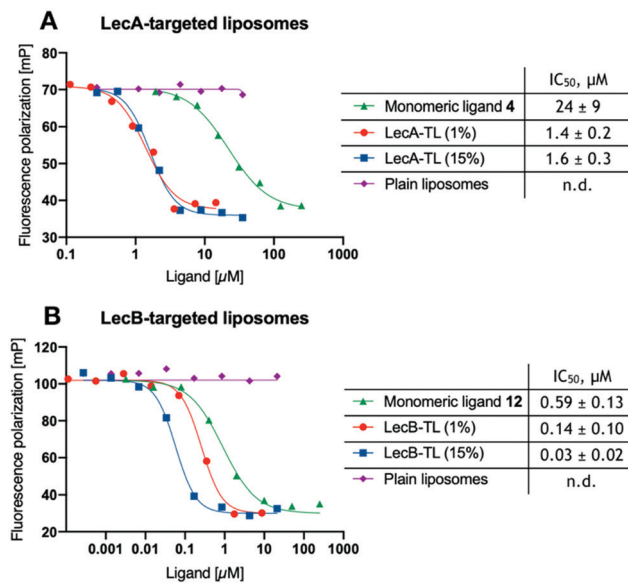
Fig. 1 Competitive binding of lectin-targeted liposomes to LecA (A) or LecB (B). Plain liposomes do not contain targeting ligand and have therefore been used at total lipid concentrations comparable to the targeted liposomes (TL). IC 50 s for liposomes are normalized and depicted per targeting group, i.e. the affinity of a liposome carrying several copies of the targeting ligand is much higher. Averages and standard deviations from at least 3 independent experiments of technical triplicates each.
