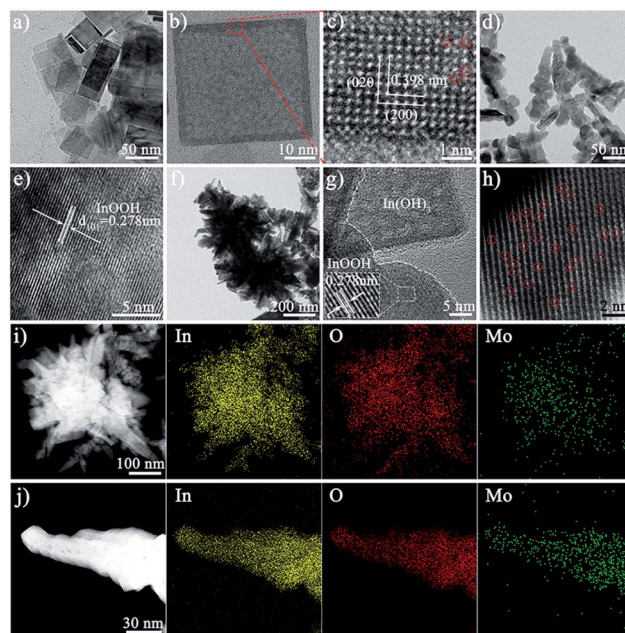
Fig. 1 (a–c) TEM and HRTEM images of \text{In}(\text{OH})_3 . (d and e) TEM and HRTEM images of \text{InOOH} . (f–h) TEM, HRTEM, and AC HAADF-STEM images of Mo- \text{InOOH}/\text{In}(\text{OH})_3 . (i and j) The HAADF-STEM image and EDX elemental mappings of Mo- \text{InOOH}/\text{In}(\text{OH})_3 with low magnification and high magnification, respectively.
