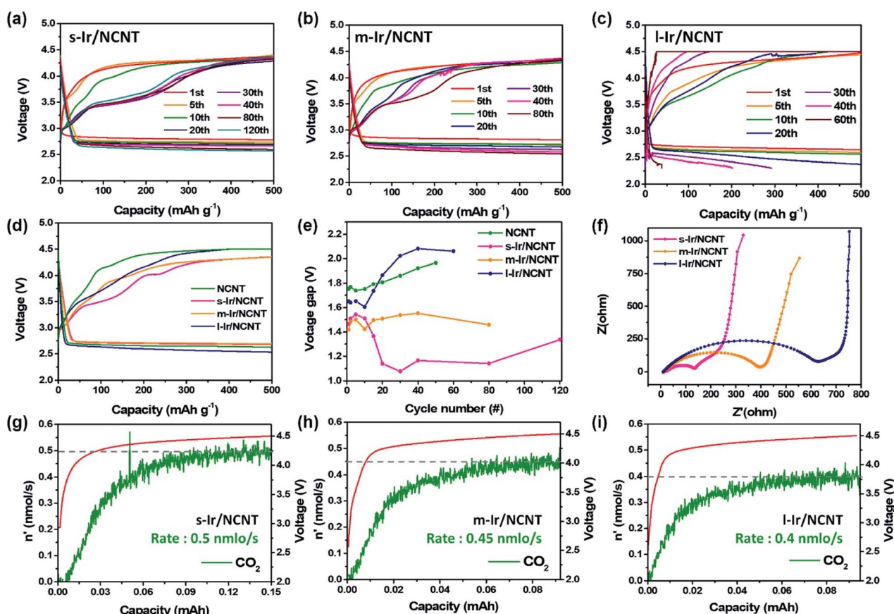
Fig. 5 Electrochemical cell data of NCNTs and s-, m- and l-Ir/NCNTs: (a–c) cycling performance of Li- \text{CO}_2 cells fabricated using s-, m-, and l-Ir/NCNTs loaded electrodes measure at 50 \text{ mA g}_{\text{carbon}}^{-1} with a limited capacity of 500 \text{ mA h g}_{\text{carbon}}^{-1} . (d) Discharge/charge curves during the 15th cycle. (e) Voltage gap graphs calculated during the discharge and charge reactions for Li- \text{CO}_2 cells at 250 \text{ mA h g}^{-1} during each cycle. (f) EIS profiles of the s-, m- and l-Ir/NCNT-containing electrode after 10 cycles. (g–i) in situ DEMS results of the gas evolution rate for \text{CO}_2 during charging in cells with s-, m- and l-Ir/NCNTs.
