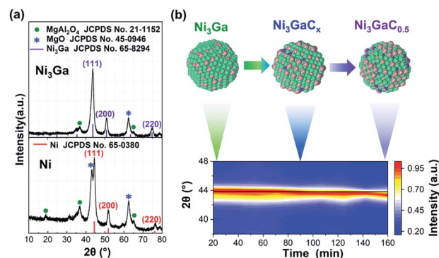
Fig. 1 (a) XRD patterns of Ni and \text{Ni}_3\text{Ga} catalysts. (b) Time-resolved XRD contour maps of the \text{Ni}_3\text{Ga} catalyst under 1.0% \text{C}_2\text{H}_2/\text{N}_2 at 300 °C, where the schematic diagram of the phase transformations from the intermetallic \text{Ni}_3\text{Ga} phase into the \text{Ni}_3\text{GaC}_{0.5} phase is shown in the inset.
