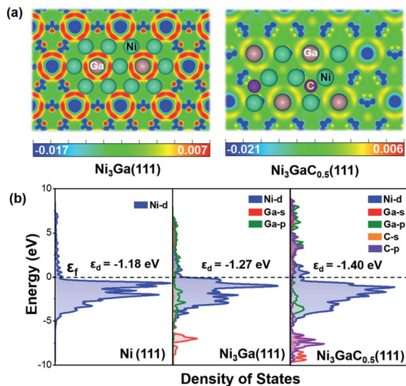
Fig. 4 (a) Two dimensional contours of the charge density difference of \text{Ni}_3\text{Ga}(111) and \text{Ni}_3\text{GaC}_{0.5}(111) surfaces, where the units of the color bars are \text{e bohr}^{-3} . (b) Projected electronic densities of states of the C p and s orbitals, Ga p and s orbitals, and those of the Ni d orbitals on \text{Ni}(111) , \text{Ni}_3\text{Ga}(111) and \text{Ni}_3\text{GaC}_{0.5}(111) surfaces.
