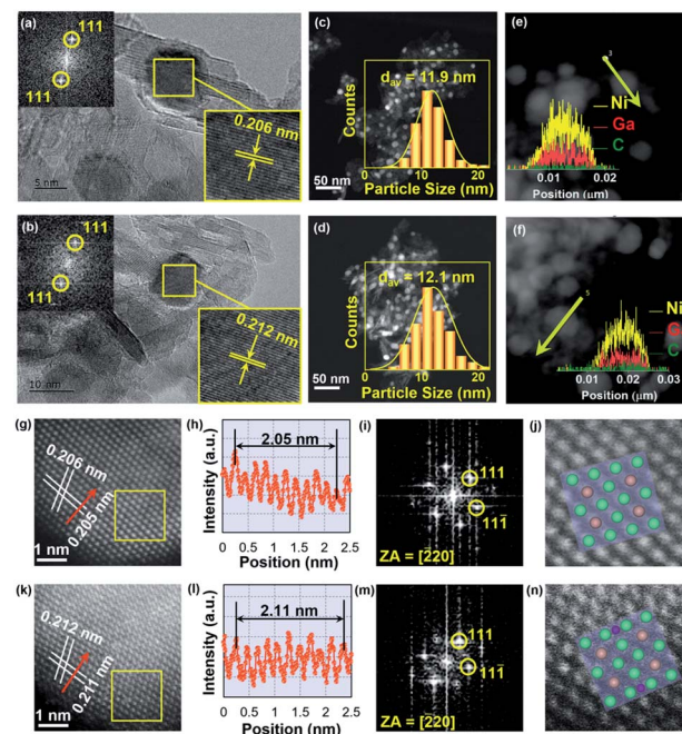
Fig. 2 HRTEM images of (a) \text{Ni}_3\text{Ga} and (b) \text{Ni}_3\text{GaC}_{0.5} catalysts. The insets are the corresponding FFT patterns. HAADF-STEM images of (c) and (e) \text{Ni}_3\text{Ga} and (d) and (f) \text{Ni}_3\text{GaC}_{0.5} catalysts. Insets in (c) and (d) are the corresponding histograms of the particle size distributions, and those in (e) and (f) are the corresponding EDS line-scanning profiles. (g) Representative AC-HAADF-STEM images of the \text{Ni}_3\text{Ga} catalyst. (h) Line intensity profiles along the direction marked by the red arrows in (g). (i) FFT patterns of the \text{Ni}_3\text{Ga} catalyst. (j) Enlarged views of the areas marked by the yellow rectangles in (g) and the corresponding crystal structure models along with [220] zones. (k) Representative AC-HAADF-STEM images of the \text{Ni}_3\text{GaC}_{0.5} catalyst. (l) Line intensity profiles along the direction marked by the red arrows in (k). (m) FFT patterns of the \text{Ni}_3\text{GaC}_{0.5} catalyst. (n) Enlarged views of the areas marked by the yellow rectangles in (k) and the corresponding crystal structure models along with [220] zones.
