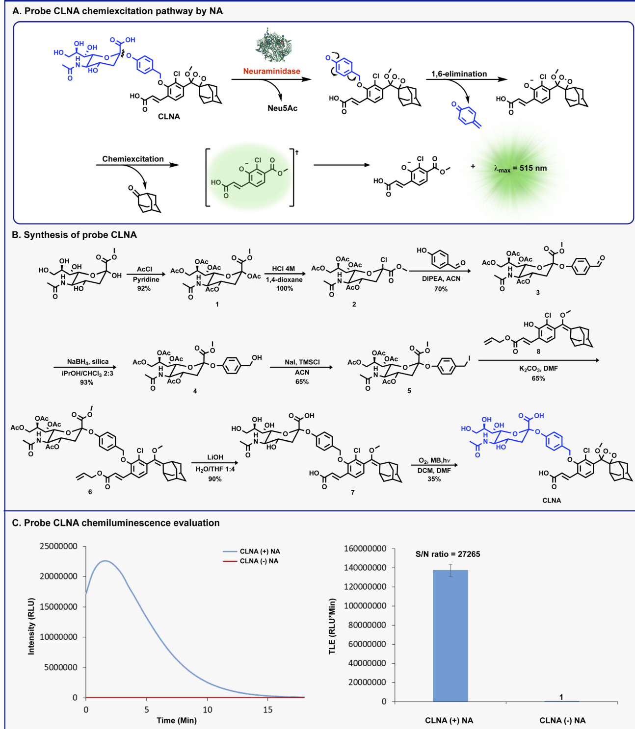
Fig. 2 (A) Chemiexcitation disassembly pathway of CLNA upon reaction with neuraminidase. (B) Chemical synthesis of probe CLNA. (C) Chemiluminescence kinetic profile (left) and total light emitted (right) obtained by CLNA [10 \mu M] in 10% DMSO in PBS pH 7.4 at 27 ^{\circ} C with and without C. perfringens neuraminidase [0.1 U mL ^{-1} ].
