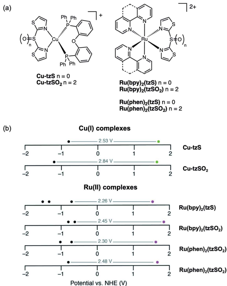
Fig. 19 (a) Structures of Cu-tzSO n and Ru(bpy) 2 (tzSO n ) and Ru(phen) 2 (tzSO n ) complexes reported by our group ( n = 0, 2). (b) Redox potentials of Cu(I) and Ru(II) complexes with reductive (black dots) and oxidative (green or purple dots) potentials illustrated. Adapted with permission from ref. 95. Copyright 2019 Royal Society of Chemistry.
