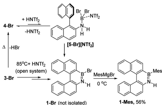
Scheme 2 Formation of 1-Br using \text{HNTf}_2 and heating in an open system (termed route i) and subsequent transformation into 1-Mes .
