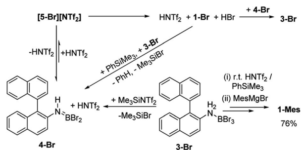
Scheme 3 \text{Me}_3\text{SiNTf}_2 mediated, N-directed, C–H borylation (termed route ii).
