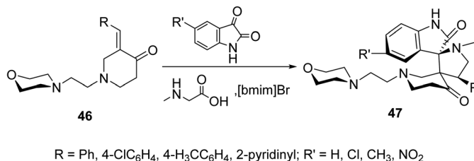
Scheme 20 Synthetic route towards spiro-piperidones 47.
