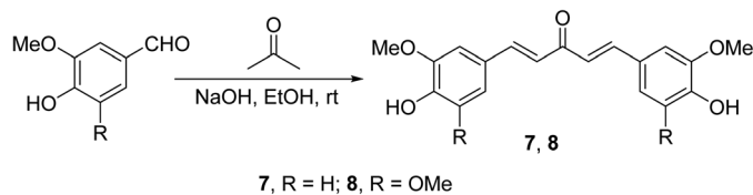
Scheme 3 Curcumin analogs 7 and 8.
