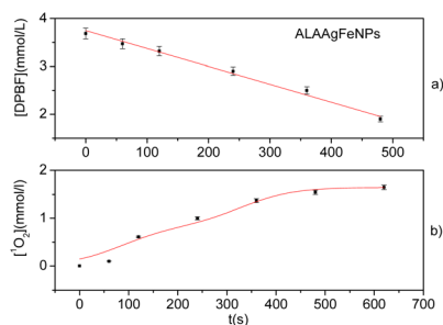
Fig. 3 (a) DPBF consumption by irradiation with LED ( 590 \pm 10 nm) of ALAAgFeNPs. DoseResp fit. (b) The quantity of ^1O_2 generated by irradiation in the function of the time for ALAAgFeNPs. BiDoseResp Fit. The data by UV-vis measurements and performed in triplicate.
