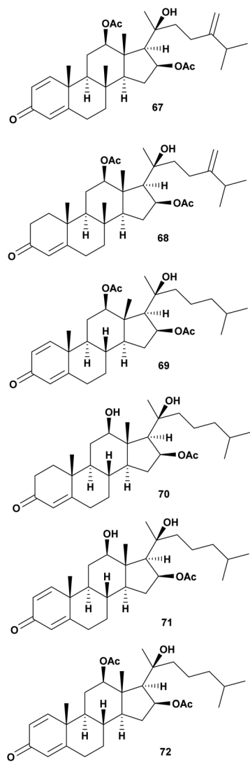
Fig. 7 Antivibrio compounds isolated from coral.
