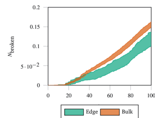
(e) Damage over time for a network with a hole of size five, tracking bonds on the edge of the hole against bonds (“edge”) against bonds away from the hole (“bulk”).
