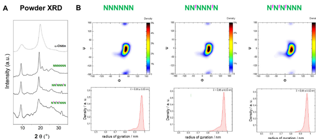
Fig. 7 (A) Powder XRD profiles of 6F-chitin compared to α-chitin profile (dotted line). (B) Ramachandran plots for all glycosidic linkages combined (top) and radius of gyration plots (bottom) extracted from the MD simulations.
