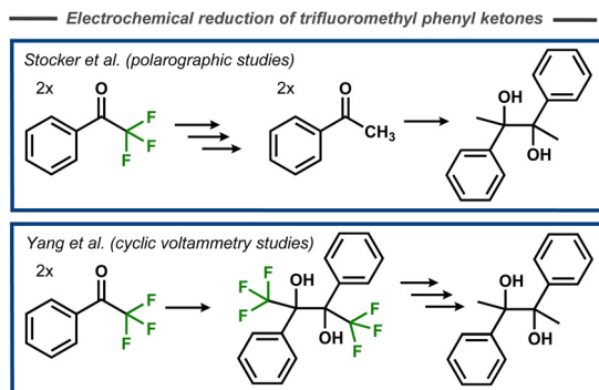
Fig. 19 Electroreductive \alpha,\alpha,\alpha -trifluoroacetophenone. 70,71
