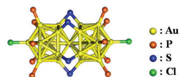
Scheme 1 Crystal structure of [Au 25 (PPh 3 ) 10 (SR) 5 Cl 2 ] 2+ . 8
