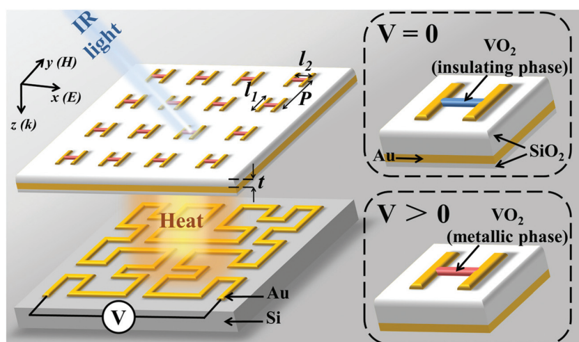
Fig. 1 Schematic drawing and tuning mechanism of MEMS-based MPA design. The periods of unit cells are kept as P = 2.3 \mu\text{m} .
