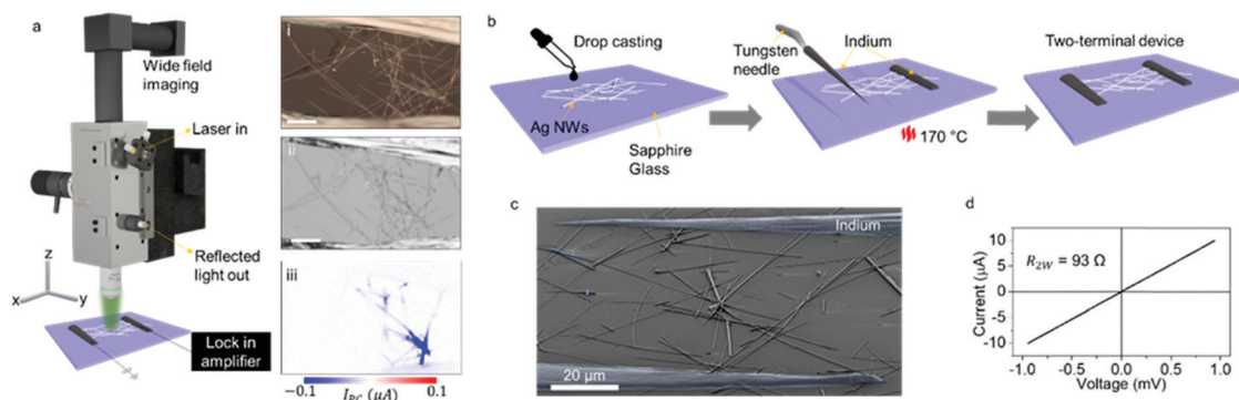
Fig. 1 (a) Schematic of our SPCM setup: The continuous-wave laser beam focused on a diffraction-limited spot raster-scans the device. (i) The wide field reflection image, (ii) reflected light intensity map and (iii) generated photocurrent map of a typical device given in the panels on the right. The scale bars are 20 \mu\text{m} . (b) The device fabrication steps depicted: Ag NWs in IPA solution are drop-cast on a sapphire or glass substrate. The substrate with Ag NWs is heated to 170 °C and indium needles are placed over the nanowire network using a micromanipulator. Upon cooling, the device is ready for two-terminal electrical and scanning photocurrent measurements. (c) False-color SEM image of a typical device: Indium needles are shaded with blue. (d) Current vs. voltage graph showing the 2-wire resistance, R_{2W} , of a typical device.
