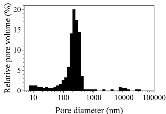
Fig. 8 Pore size distribution histogram obtained from mercury intrusion porosimetry data of S-sintered COK-12 monoliths processed at 12.5 MPa and 800 °C.
