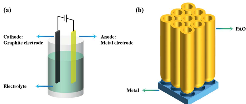
Fig. 1 (a) Anodizing device; (b) PAO array.
