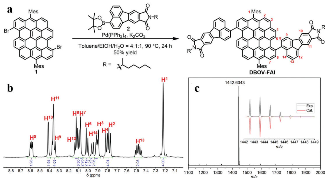
Fig. 1 (a) Synthetic route towards DBOV-FAI; (b) aromatic region of the ^1\text{H} NMR spectrum of DBOV-FAI in \text{C}_2\text{D}_2\text{Cl}_4 : \text{CS}_2 = 2 : 1 (500 MHz, 303 K); (c) high-resolution MALDI-TOF MS spectrum of DBOV-FAI (inset shows comparison of the experimental isotopic distribution pattern with the simulated pattern for \text{C}_{106}\text{H}_{78}\text{N}_2\text{O}_4 ).
