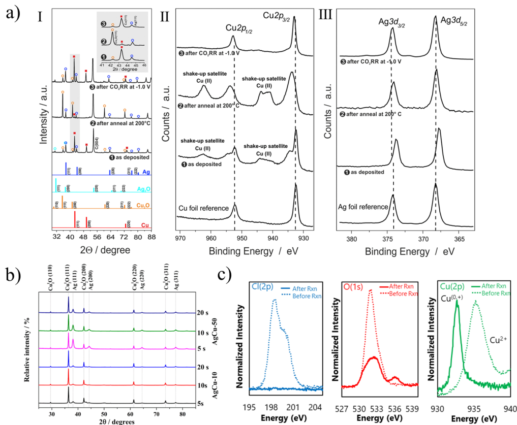
Fig. 8 (a) (I) XRD patterns of the as deposited \text{Ag}_{15}\text{Cu}_{85} foam, the annealed foam (12 h at 200 °C), and OD- \text{Ag}_{15}\text{Cu}_{85} (after 1 h \text{CO}_2 RR at -1.0 V vs. RHE); (II and III) corresponding XPS of the bimetallic foam. Reproduced with permission. 59 Copyright 2020, Elsevier. (b) XRD patterns of AgCu film electrodeposited. Reproduced with permission. 48 Copyright 2019, American Chemical Society. (c) XPS spectra of electro-redeposited (ERD) copper before and after the reaction. Reproduced with permission. 49 Copyright 2018, Macmillan Publishers Limited.
