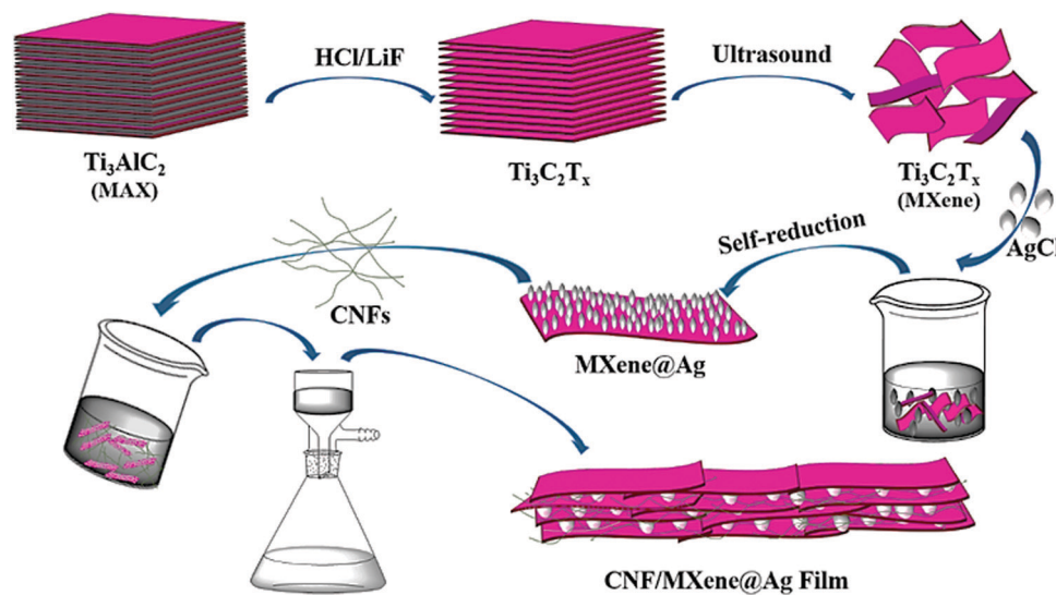
Fig. 1 Preparative process for cellulose nanofibers (CNF)/MXene@Ag multifunctional films with unique photothermal and mechanical features. Reproduced with permission from ref. 56 Copyright 2021 Elsevier.
