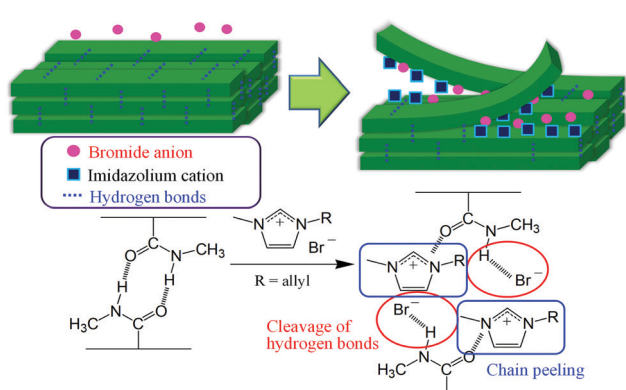
Fig. 5 Plausible dissolution process of chitin in AMIMBr predicted by molecular dynamics (MD) simulations.
