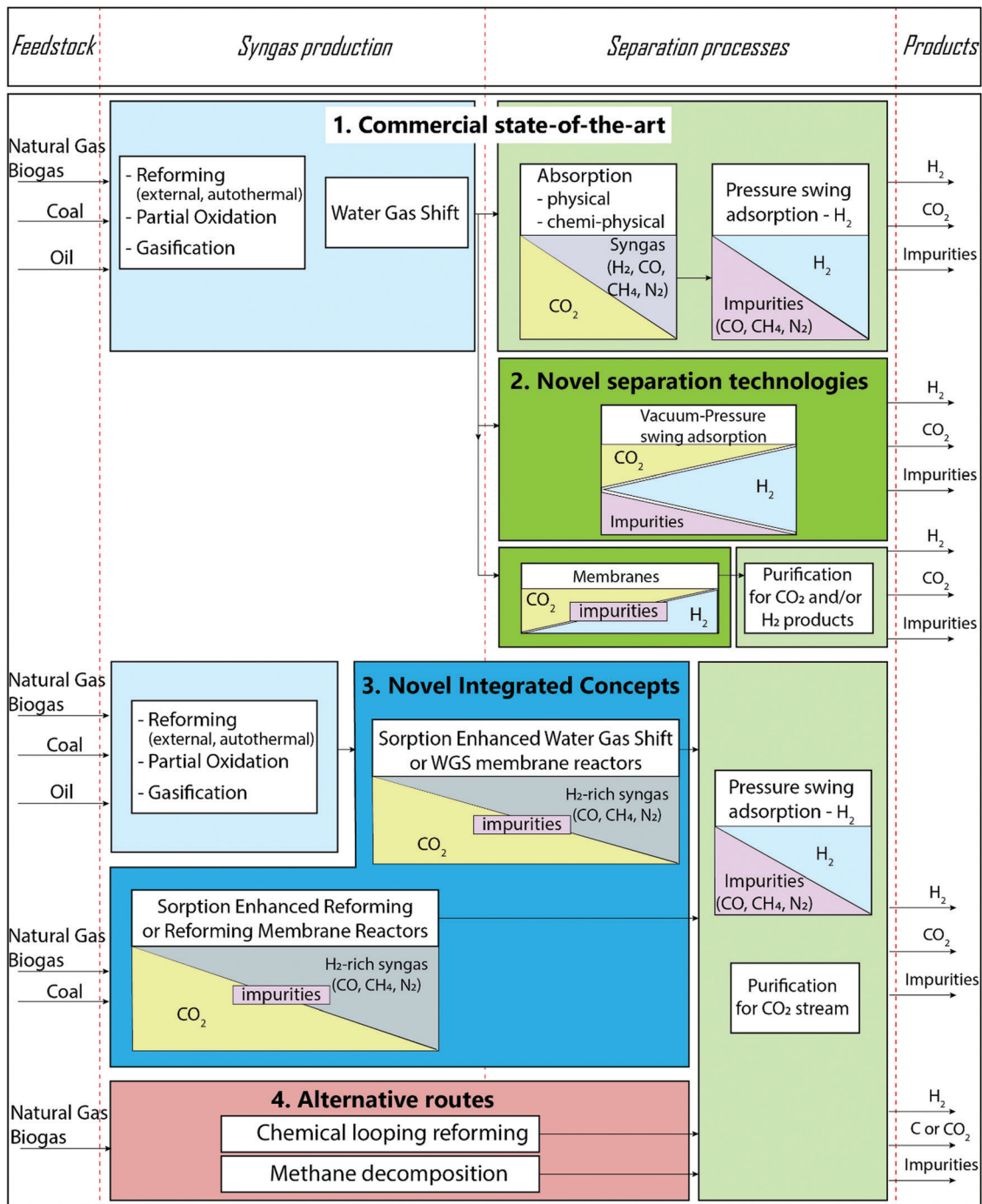
Fig. 9 Hydrogen production from fossil fuels with carbon capture and storage, with highlight on current and future pathways relevant for \text{CO}_2 -neutrality in 2050.
