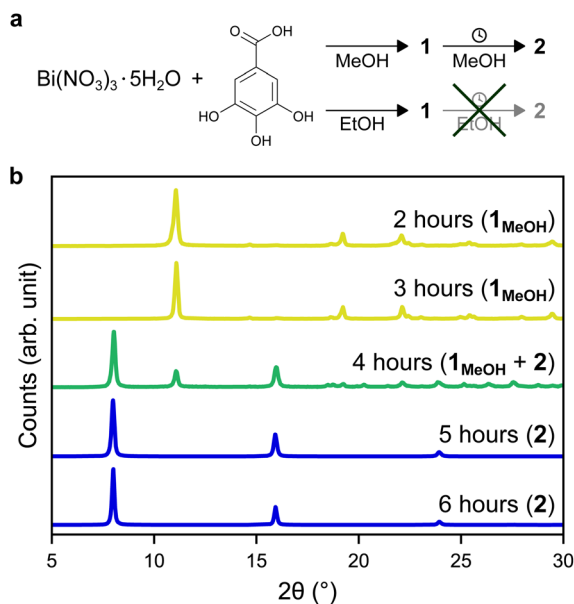
Fig. 1 (a) Schematic representation of the synthesis of 1 MeOH / 1 EtOH from Bi(NO 3 ) 3 ·5H 2 O and gallic acid in methanol/ethanol, where 1 MeOH transforms into 2 upon continued heating in methanol. (b) X-ray powder diffraction patterns of bismuth gallates synthesized in methanol under identical conditions apart from different synthesis times. At short reaction times the MOF 1 MeOH forms, which after a synthesis time of 4 hours begins to convert into the layered phase, 2 .
