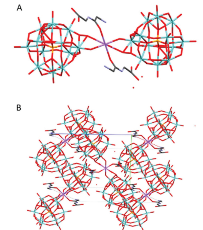
Fig. 7 The molecular (A) and crystal (B) structure of compound Na(HGlyGly) 2 (H 3 O) 3 [PMo 12 O 40 ] 2 ·3H 2 O (7).
