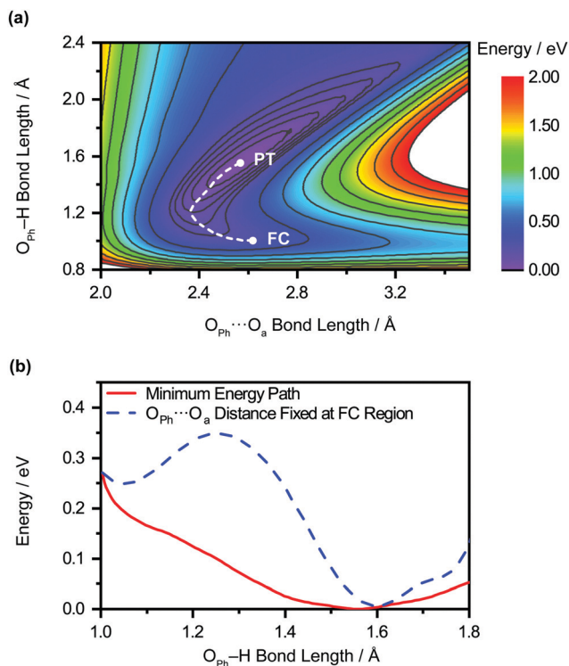
Fig. 4 (a) 2D PES for the PT of the microhydrated phenol radical cation, \text{PhOH}^{\bullet+}-(\text{H}_2\text{O})_5 , as a function of \text{O}_{\text{Ph}}\cdots\text{O}_a and \text{O}_{\text{Ph}}-\text{H} distances. The locations of the Franck-Condon region and the proton transfer product are denoted "FC" and "PT", respectively, and the connecting minimum energy path is represented by the dashed line. (b) Potential energy curves of \text{PhOH}^{\bullet+}-(\text{H}_2\text{O})_5 as a function of \text{O}_{\text{Ph}}-\text{H} distance along the minimum energy path (red solid line) and where the \text{O}_{\text{Ph}}\cdots\text{O}_a distance is fixed at that of the Franck-Condon region (blue dashed line).
