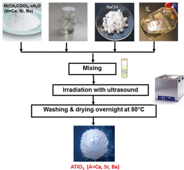
Fig. 10 Sonochemical ambient condition preparation of perovskite photocatalysts.
