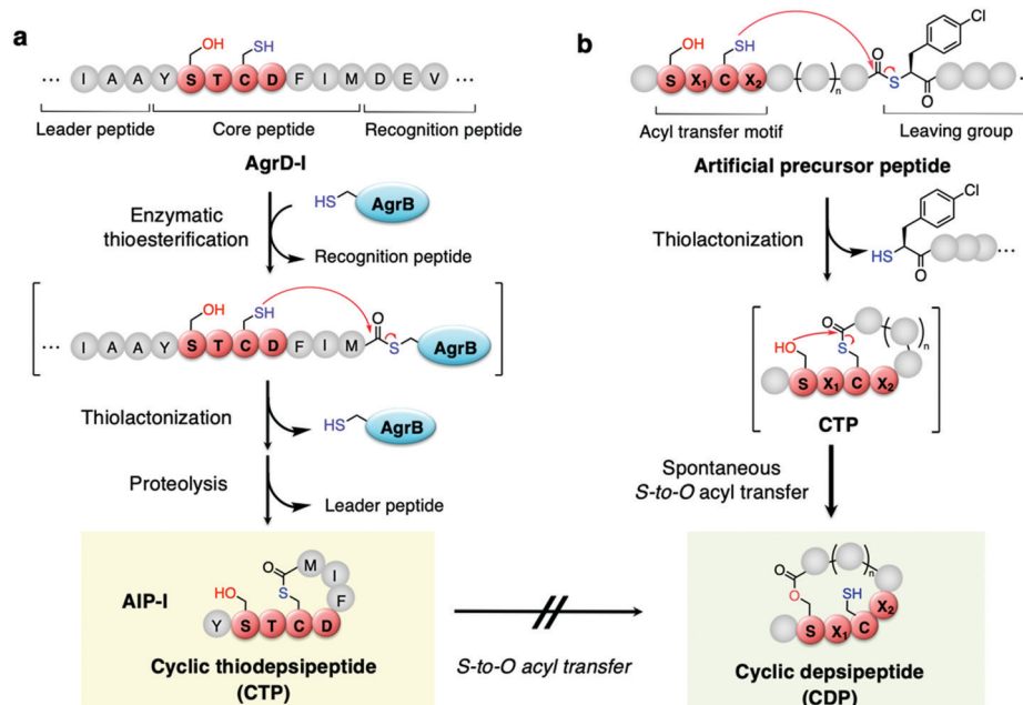
Fig. 1 Ribosomal synthesis of cyclic thiopeptides (CTPs) possessing an SX_1CX_2 motif and a downstream thioester. (a) Biosynthesis of autoinducing peptide I (AIP-I) from AgrD-I as a precursor peptide. (b) One-pot in vitro ribosomal cyclic depsipeptide (CDP) synthesis. In this case a CTP acts as an intermediate and is spontaneously converted to CDP via an S-to-O acyl transfer modulated by an SX_1CX_2 motif. N \geq 1 , depending on the X_2 residue.
