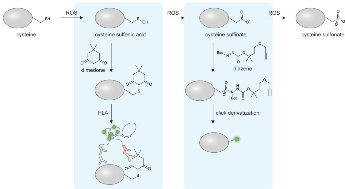
Fig. 6 Detection of non-enzymatic oxidative proteoforms. The thiol group of cysteine can be oxidized sequentially to sulfenic acid, sulfinate, and sulfonate. Sulfenylated cysteines can be chemically derivatized with dimedone, the product of which can be detected with an antibody. Sulfenylated cysteines can be derivatized with electrophilic diazene compounds to install bioorthogonal functional groups and/or fluorophores. ROS, reactive oxygen species.
