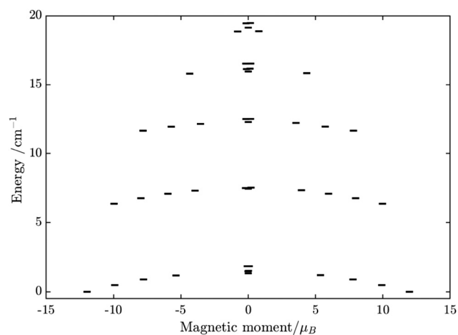
Fig. 7 Calculated low-lying spin-orbit manifolds of states arising from the magnetic interaction between the ground multiplet S = 5/2 of the \text{Fe}^{\text{III}} ion and the ground term {}^8\text{S} of the \text{Gd}^{\text{III}} ion in the [\text{Fe}^{\text{III}}\text{Gd}^{\text{III}}] complex. The components of each doublet (black lines) are placed on the diagram according to their magnetic moment projection on the main magnetic axis of the ground doublet (with energy zero).
