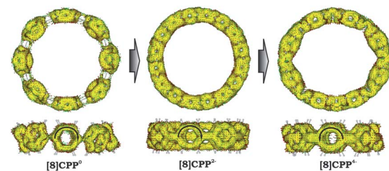
Fig. 10 \pi -Contribution to the ACID isosurface for 0 , 2- , and 4- (PBE0/cc-pVTZ). Current density vectors are plotted onto the ACID isosurface to indicate diatropic and paratropic ring currents.
