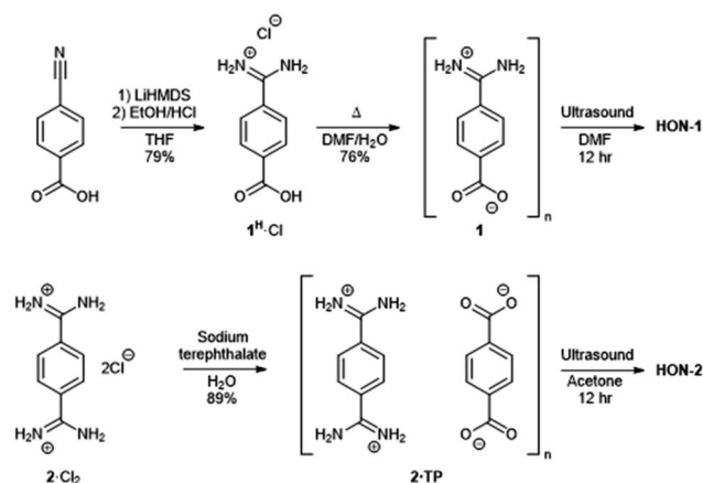
Fig. 1 Scheme showing the synthesis of hydrogen-bonded frameworks 1 and 2·TP and their exfoliation to form HON-1 and HON-2.
