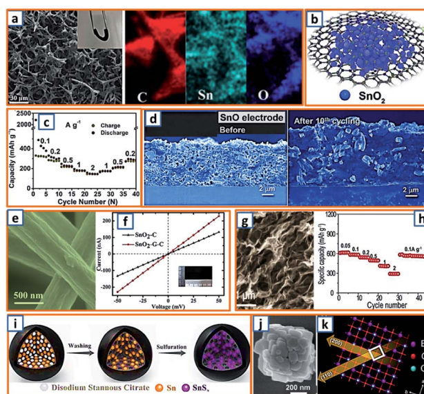
Fig. 14 Potassium storage chemistry and applications of anodes with a conversion–alloy mechanism. (a) SEM images and elemental mapping of SnO 2 @CF with the photograph of the freestanding SnO 2 @CF inserted. Reproduced with permission. 16 Copyright 2020, The Royal Society of Chemistry. (b) Schematic illustration of the 3D SnO 2 @C and (c) its corresponding rate performance. Reproduced with permission. 41 Copyright 2019, Elsevier. (d) SEM of the SnO electrode before and after cycling without cracks recognized. Reproduced with permission. 59 Copyright 2018, American Chemical Society. (e) Morphology of SnO 2 –G–C nanofibers and (f) its electrical conductivity measurement. Reproduced with permission. 74 Copyright 2018, Elsevier. (g) Morphology and (h) rate capabilities of the SnS 2 /graphene nanocomposite. Reproduced with permission. 90 Copyright 2019, Elsevier. (i) Illustration of the synthesized SnS 2 @C@rGO as the anode in a KIB. Reproduced with permission. 104 Copyright 2019, Wiley. (j) SEM and (k) schematic diagram of the crystal structure of the BiOCl anode material. Reproduced with permission. 114 Copyright 2019, The Royal Society of Chemistry.
