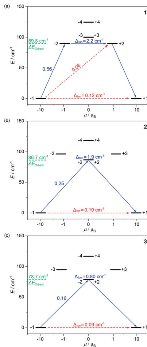
Fig. 3 The energy splitting of the ground 5\text{I}_8 multiplet of \text{Ho}^{\text{III}} in 1 (a), 2 (b), and 3 (c) obtained from the ab initio calculations. Only the lowest energy part was presented. The resulting energy barriers of the Orbach relaxation were shown in green colour. The numbers above each arrow represent the corresponding matrix element of the transversal magnetic moment while the \Delta_{\text{tun}} shows the tunnelling gap of the indicated doublets. Red arrows indicate the less possible whereas blue arrows show the most probable relaxation pathway. The scheme is obtained for the L–W models (Table S8†).
