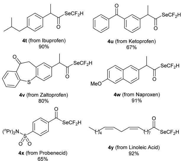
Scheme 3 Scope of the deoxydifluoromethylselenylation of carboxylic acids. Conditions: 3 (0.3 mmol), BT-SeCF 2 H (2 eq.), NaH (2 eq.) in THF (0.2 M), 45 °C, 2 h. Isolated yields. a Reactions conducted at rt.
