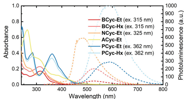
Fig. 1 UV-vis absorption (solid lines) and photoluminescence spectra (dashed lines) of the macrocycles in \text{CHCl}_3 solution ( 5\ \mu\text{M} ). The excitation wavelengths for recording the photoluminescence (PL) spectra are shown in brackets; spectra obtained at other excitation wavelengths are available (ESI Fig. S43†).
