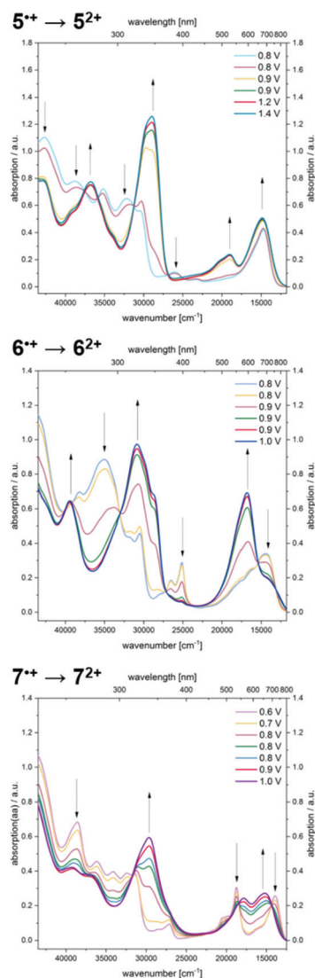
Fig. 8 UV/Vis spectroelectrochemical measurements of radical cations 5^+ , 6^+ , and 7^+ forming the corresponding dication 5^{2+} , 6^{2+} , and 7^{2+} ( \text{CH}_2\text{Cl}_2 , T = 293 K; electrolyte 0.1 M [\text{tBu}_4\text{N}][\text{PF}_6] ; Pt working electrode, Pt counter electrode and Ag/AgCl pseudo reference electrode).
