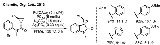
Scheme 6 Pd-Catalysed C–H arylation to form 3,3'-spirooxindoles. Cy = cyclohexane.
