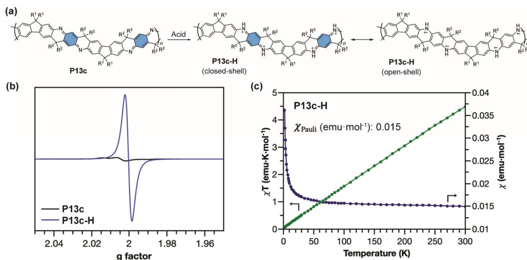
Fig. 14 (a) Structural representation of P13c and its acid-doped form P13c-H with closed-shell and open-shell resonance structures; (b) EPR spectra of P13c and P13c-H ; (c) \chi T and \chi vs T plots of P13c-H showing dominant Pauli paramagnetism. Reproduced from ref. 87 with permission from the Royal Society of Chemistry.
