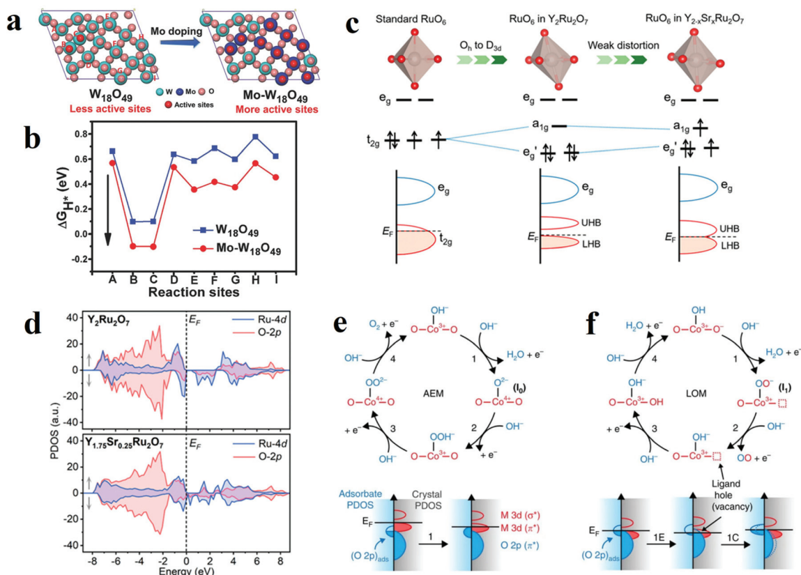
Fig. 10 (a) Different oxygen sites on W 18 O 49 (O10) and Mo-W 18 O 49 (O10). (b) The calculated Gibbs free energy of HER on different oxygen sites of W 18 O 49 (O10) and Mo-W 18 O 49 (O10). 113 (c) Schematic illustrations of different RuO 6 along with the splitting of Ru 4d orbitals. (d) Schematic evolution of band alignments through Sr 2+ substitution for Y 3+ in Y 2 Ru 2 O 7 . 127 (e and f) Relationship between oxygen vacancy concentration and Co–O bond. 115
